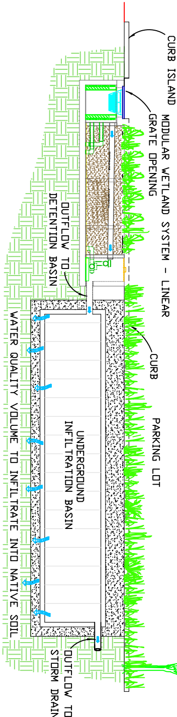
SECTION VIEW
