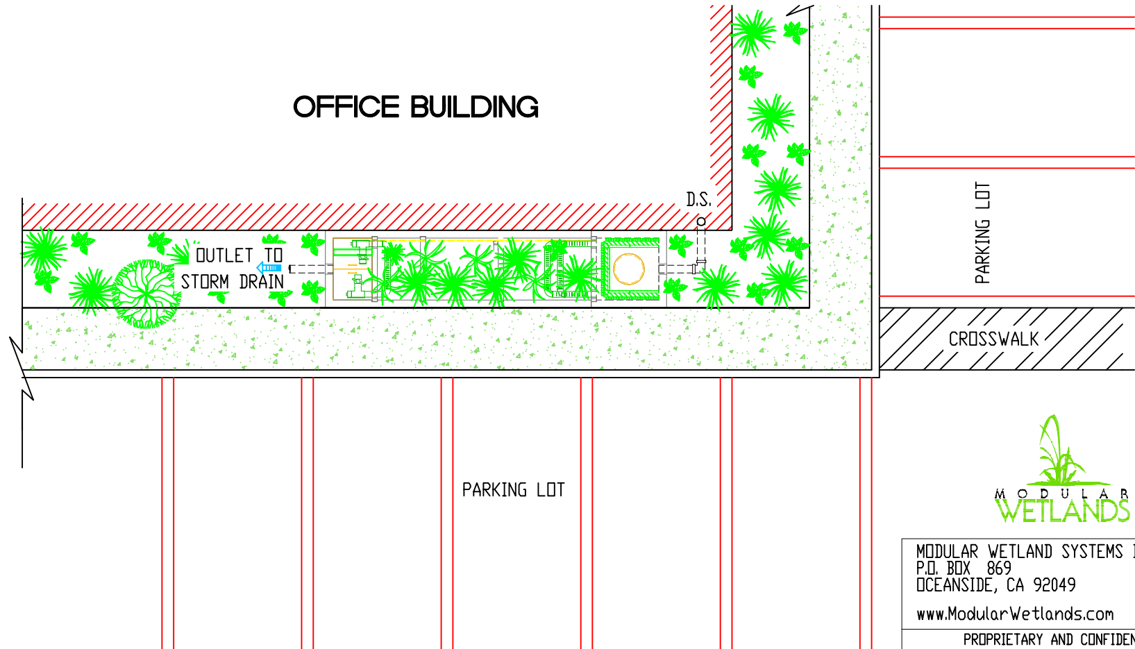
PLAN VIEW
