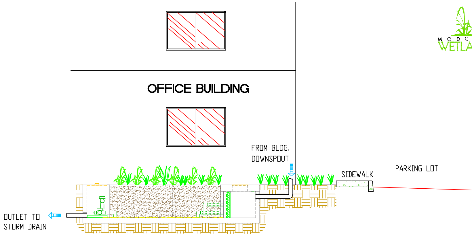
ELEVATION VIEW
